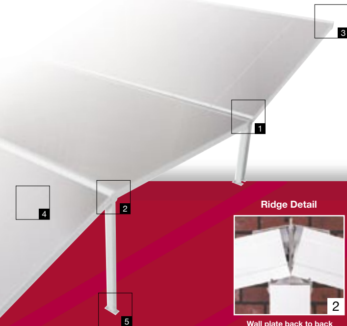
Wall plate back to back forming ridge application
